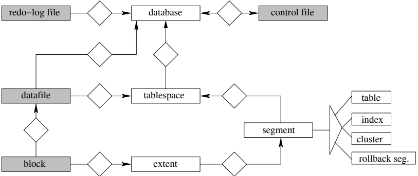
Figure 5: Relationships between logical and physical database structures
